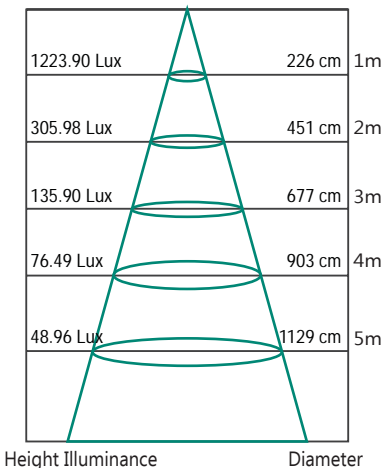
Lux Distance Curve
