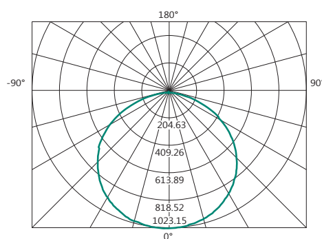
Polar Curve
