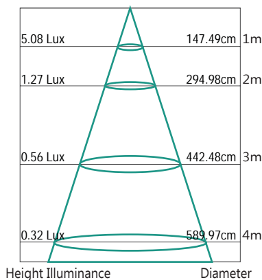
Lux Distance Curve
