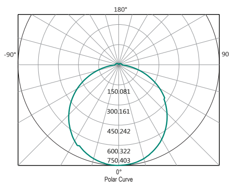
Polar Curve
