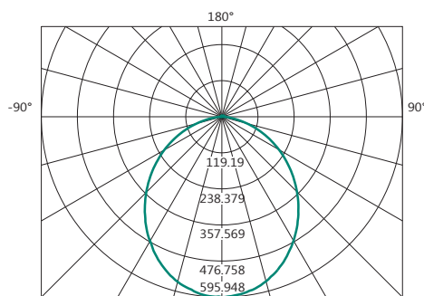
Polar Curve
