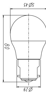
FR33 & FR37 (B22 BASE)
