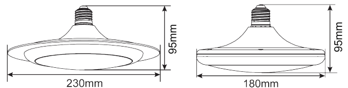
LYRA series
